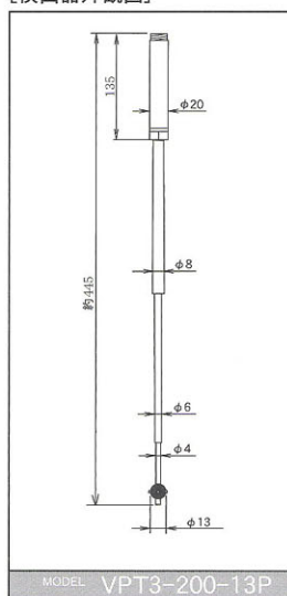
[検出器外観図]
